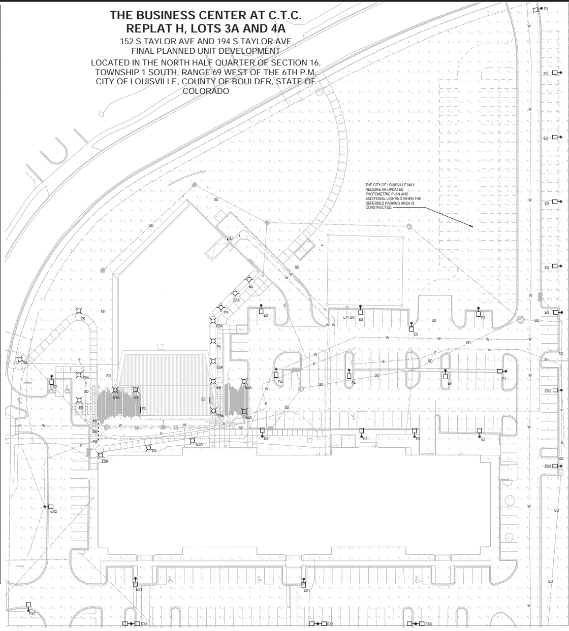
1 SITE LIGHTING AND PHOTOMETRIC PLAN 1" = 30'-0"
